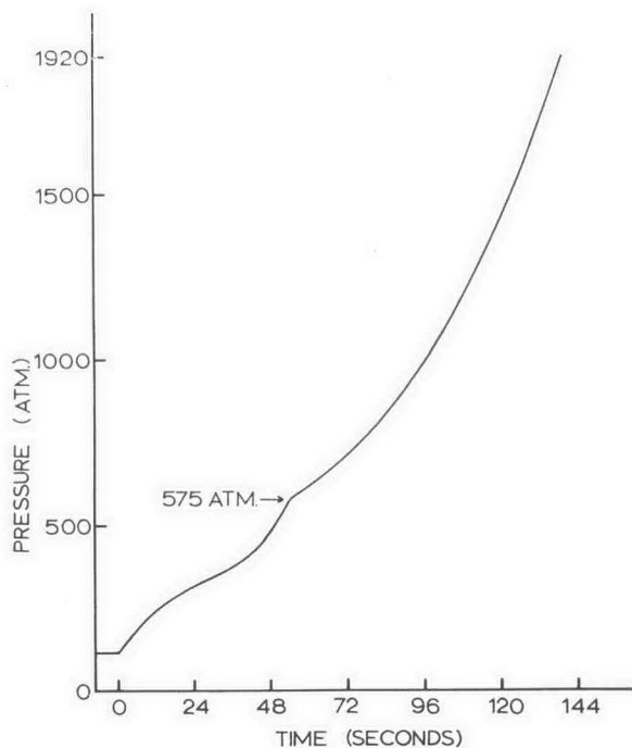
Fig. 1. Instron pressure trace at 136°C under a plunger velocity of 0.5 cm/min with a capillary of 0.0508 cm diameter, 1.55 cm length, and 90° entrance angle.
